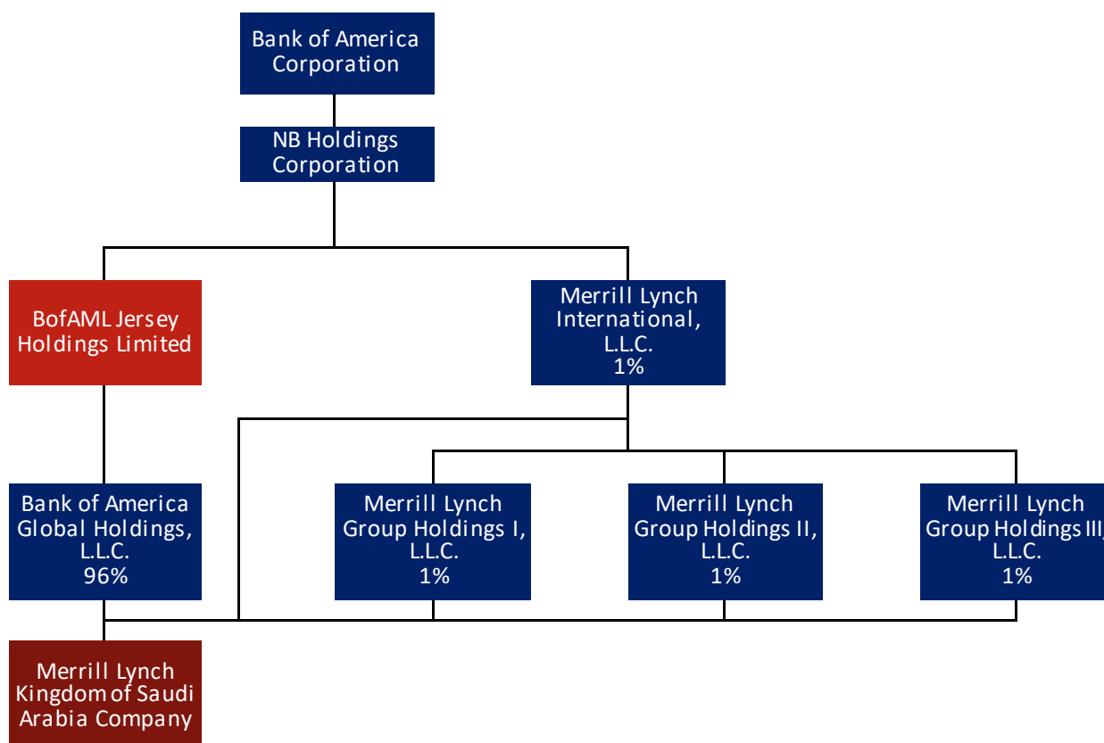
Figure 2. – Organisation Chart
